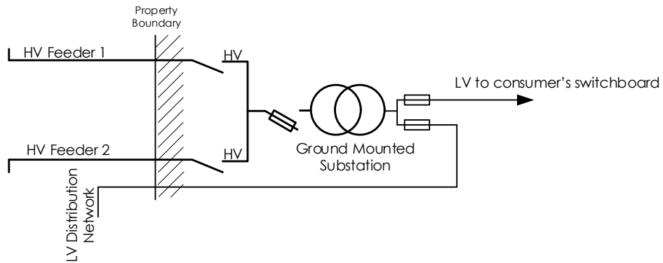
Figure 14 - Typical LV connection with HV feed-through and LV inter-connection
