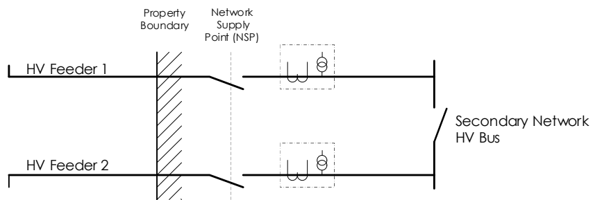
Figure 19 - HV secondary network dual-feed connection – HV metering
