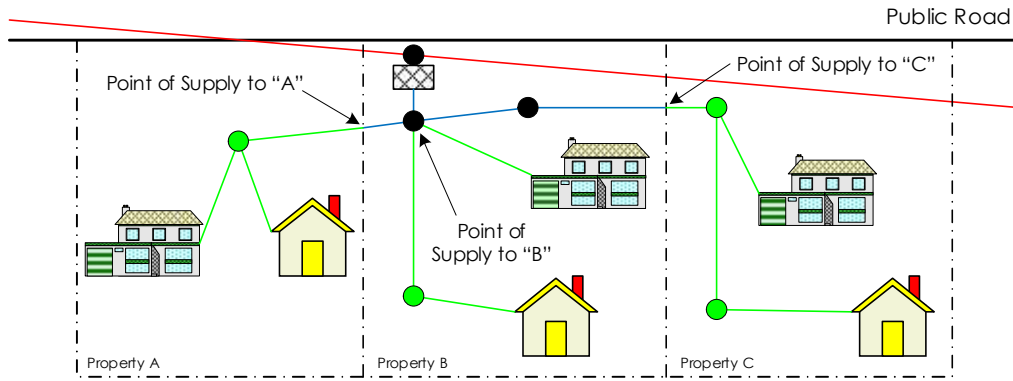
Figure 4 - Point of supply explanatory diagram 2
