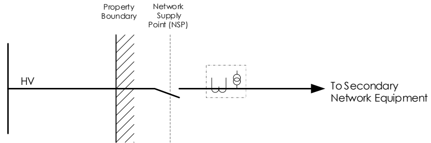
Figure 17 - HV secondary network tee connection – HV metering
