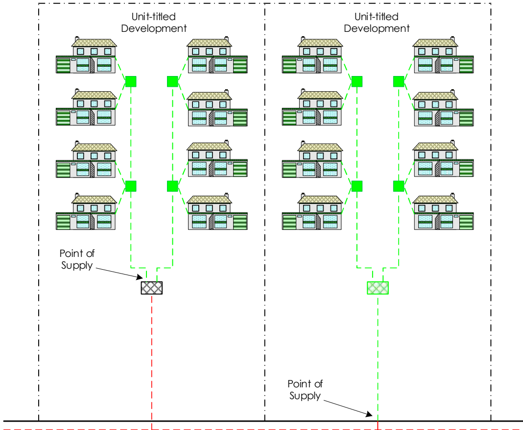
Figure 8 - Point of supply explanatory diagram 6
