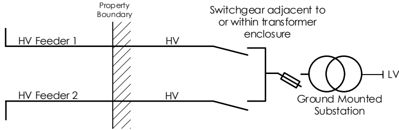
Figure 12 - Typical LV connection with HV feed-through (type 1)
