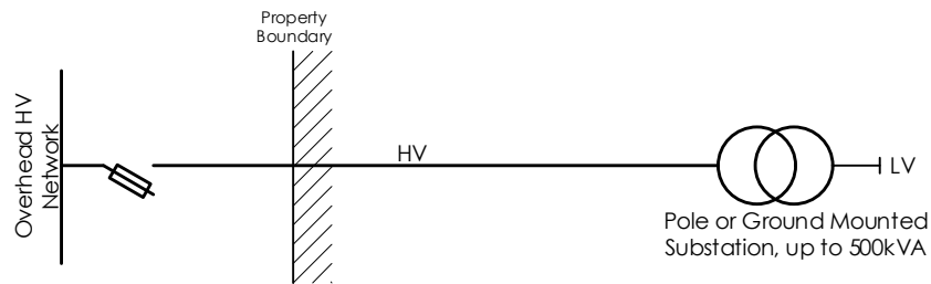
Figure 10 - Typical fused tee connection - LV supply
