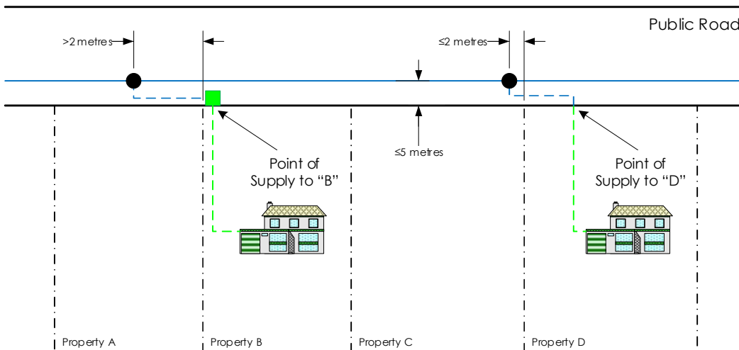
Figure 2 - Underground connections from overhead supply
