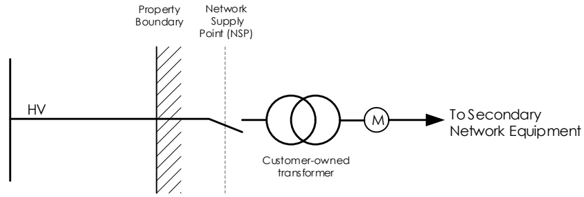
Figure 16 - HV secondary network tee connection – LV metering
