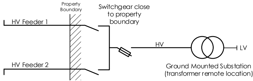
Figure 13 - Typical LV connection with HV feed-through (type 2)
