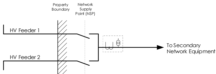
Figure 18 - HV secondary network feed-through connection – HV metering
